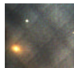
M109 galaxy 55 million light years from earth.
